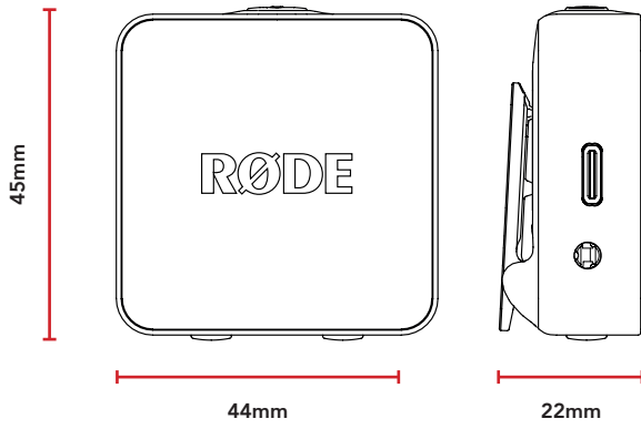
Receiver (RX)
